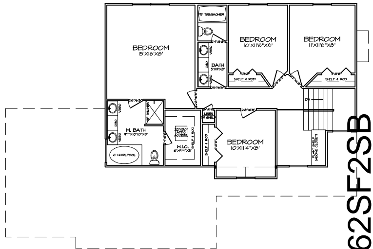
SECOND FLOOR PLAN A-5
