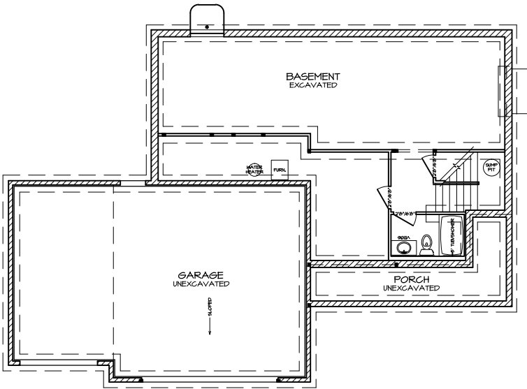
FOUNDATION PLAN A-3
